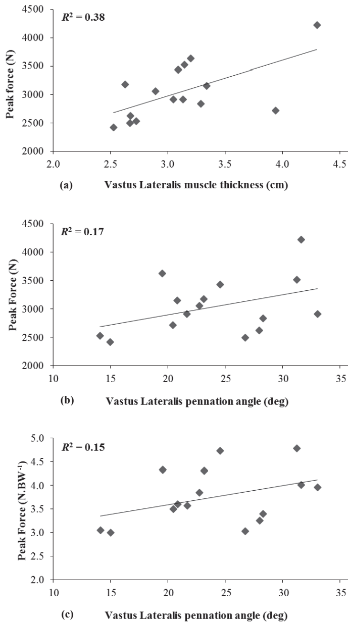
Figure 1 Relationships between (a) vastus lateralis muscle thickness and absolute isometric mid-thigh pull peak force; (b) vastus lateralis pennation angle and absolute isometric mid-thigh pull peak force; (c) vastus lateralis pennation angle and relative isometric mid-thigh pull peak force.
